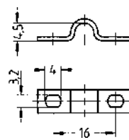
Cable diameter 5 mm
